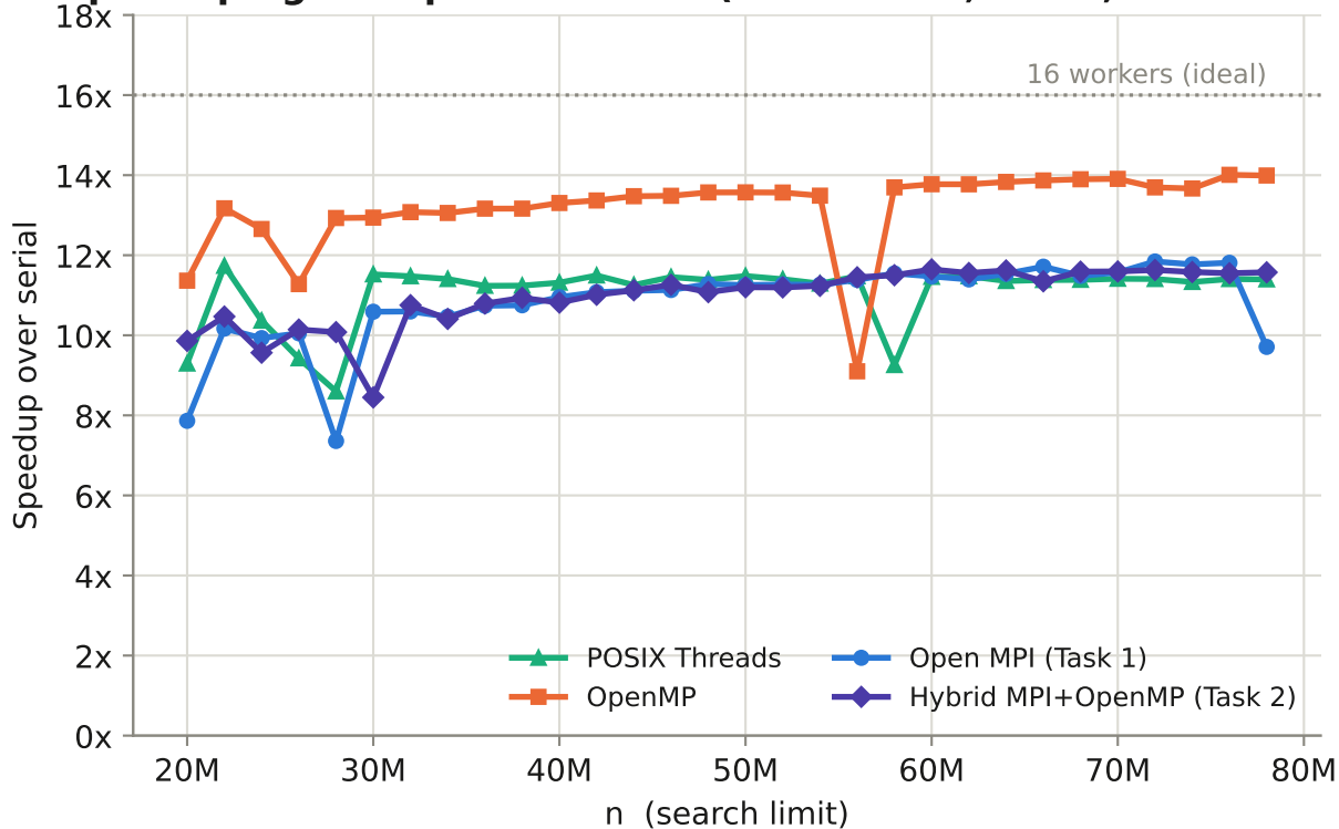
Speedup against problem size (16 workers, CAAS, median of 3)
